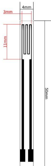
TFCH13 Thick film ceramic heater - 13Ω (ohm)
